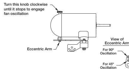
Figure 8 — Oscillating Mode
