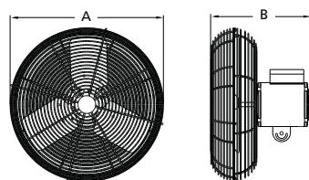
Figure 1 — Nonoscillating Dimensions
