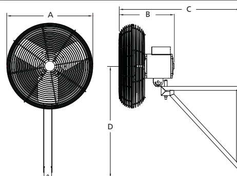
Figure 6 — 3PEH2A Dimensions
