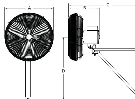
Figure 3 — 3PEG9A Dimensions
