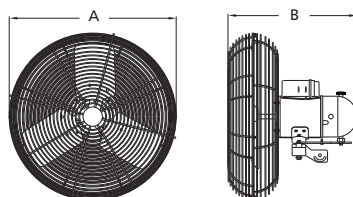
Figure 2 — Oscillating Dimensions
