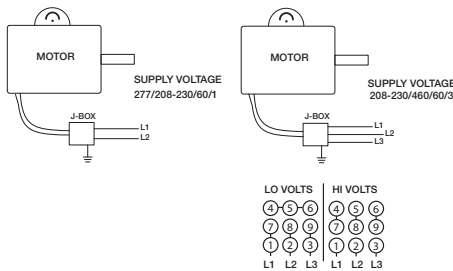
Figure 7 — Typical Wiring Diagram
